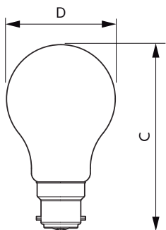
Bulb A60 EU 3.5-40W 475lm WG B22 FR
