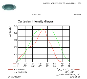
OFCC1_DBP521 1xCDM-Tm20W EB A GC +ZBP521 BSO.EPS
