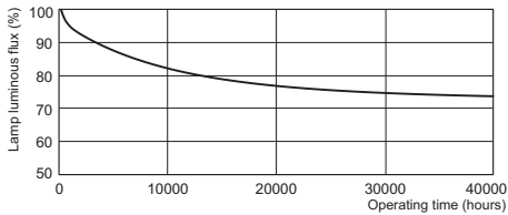
Lumen Maintenance 3 h, 12 h + 24 h cycle
