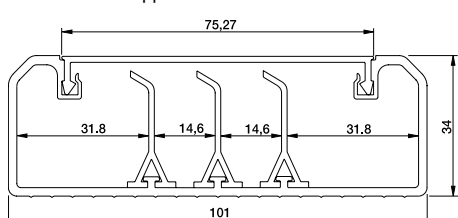
101x34 with snapped-in cable shelves
