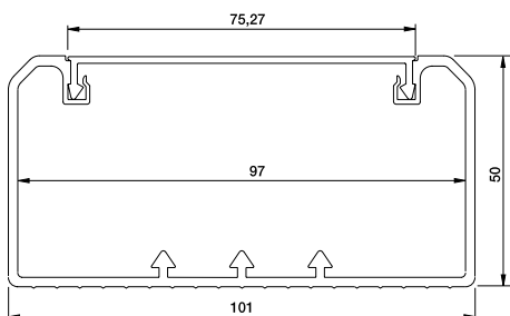
101x50 with snapped-in cable shelf
