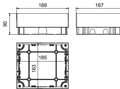
4-module screeded floor box
