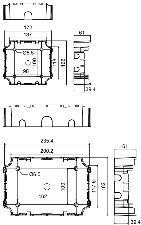
4-module and 6-module base box
