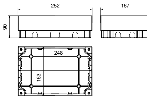
6-module screeded floor box
