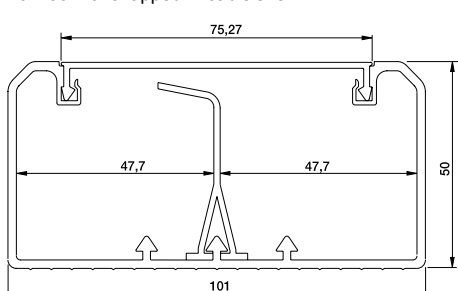
101x50 with snapped-in cable shelf
