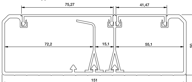
151x50 with snapped-in cable shelf
