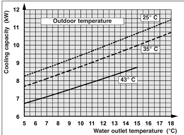
COOLING CAPACITY
