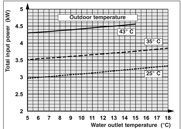
INPUT POWER
