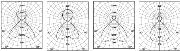
1x35 W, Beta 2x35 W, Beta 1x35 W, Lamell 2x35 W, Lamell
