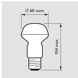
NR60 E27 Dimensions in mm
