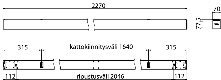
Aino Ramppi LED AIL1842F
