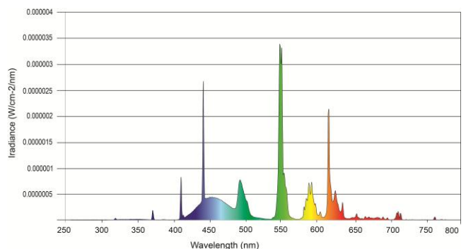
Spectral distribution 865
