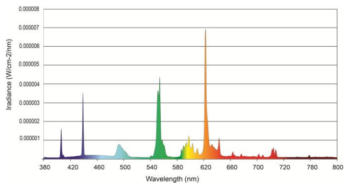
Spectral distribution 865
