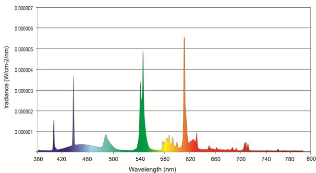
Spectral distribution 840
