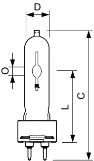
CDM-T Evol 35W/930 G12
