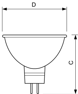
DICHRO Pro 14811 20W GU5.3 12V MR16 24D
