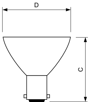
Alu 37mm 6435 20W BA15d 12V 32D CL
