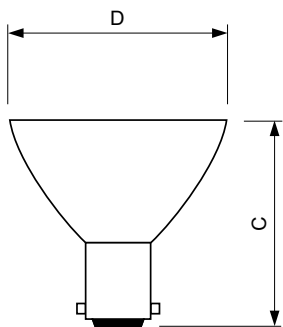
Alu 37mm 6433 20W BA15d 12V 6D CL
