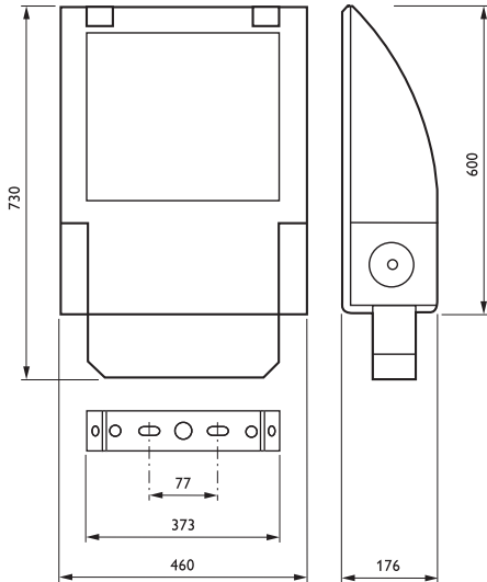
MVP506 SON-TTP400W K A GR ST
