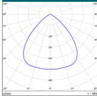
AURA CERTOS, 90° LENS OPTIC
