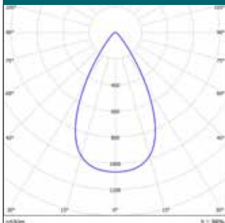
AURA CERTOS, 60° LENS OPTIC
