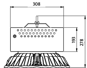
AURA CERTOS EMERGENCY
