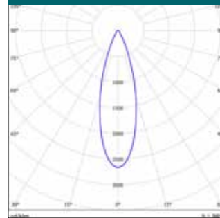
AURA CERTOS, 30° LENS OPTIC
