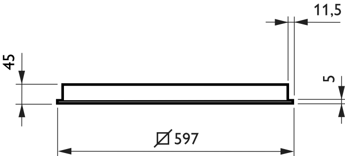
SmartForm TBS460-TBS478
