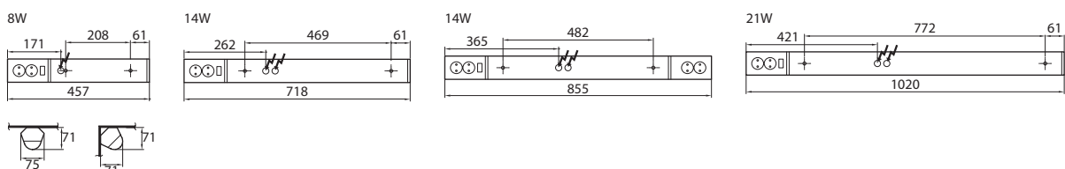
Vanamo T5
