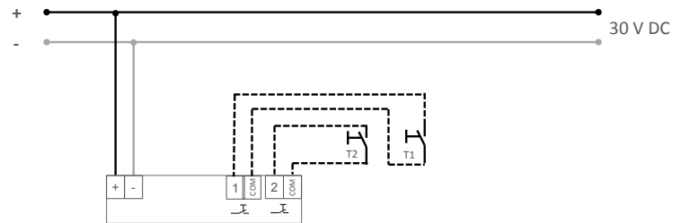
WIRE DIAGRAM KNX SYSTEM
