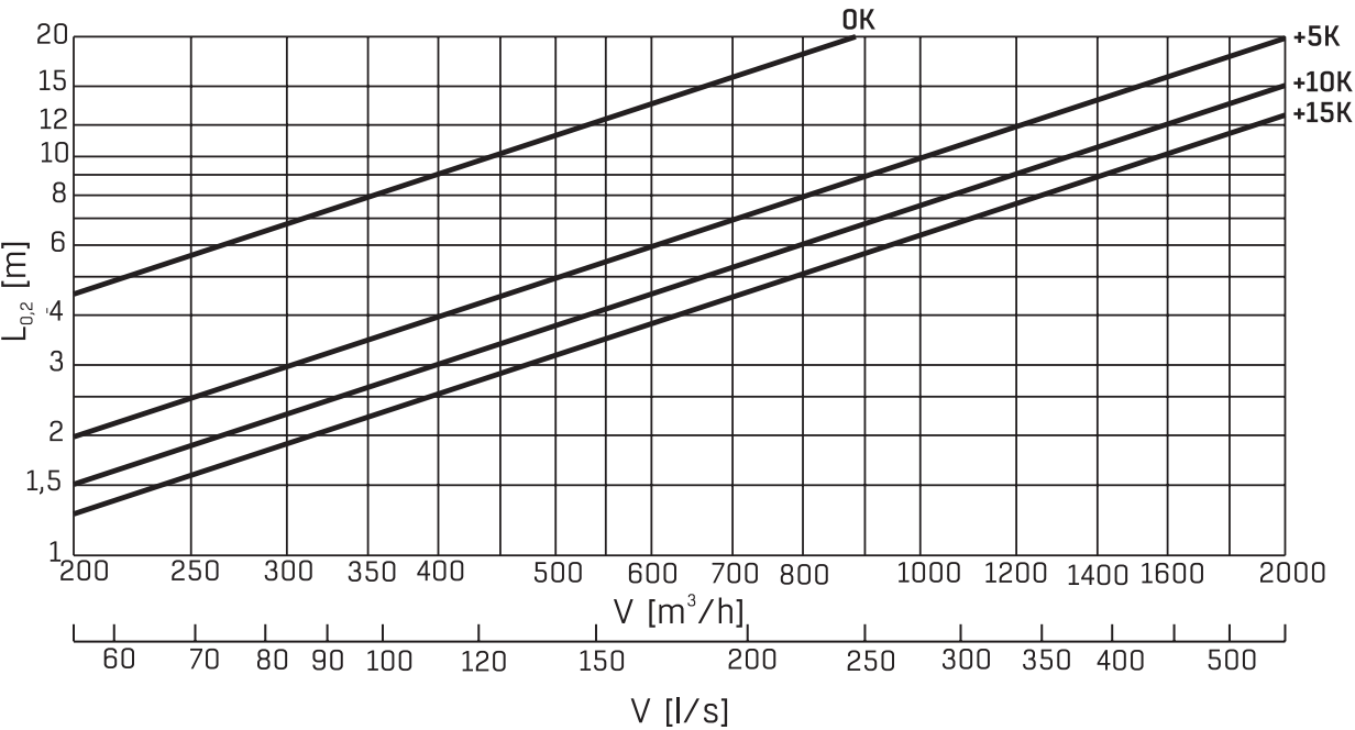
ODZA-31 – THROW LENGTH FOR HEATING FUNCTION (VERTICAL DIFFUSION PATTERN)
