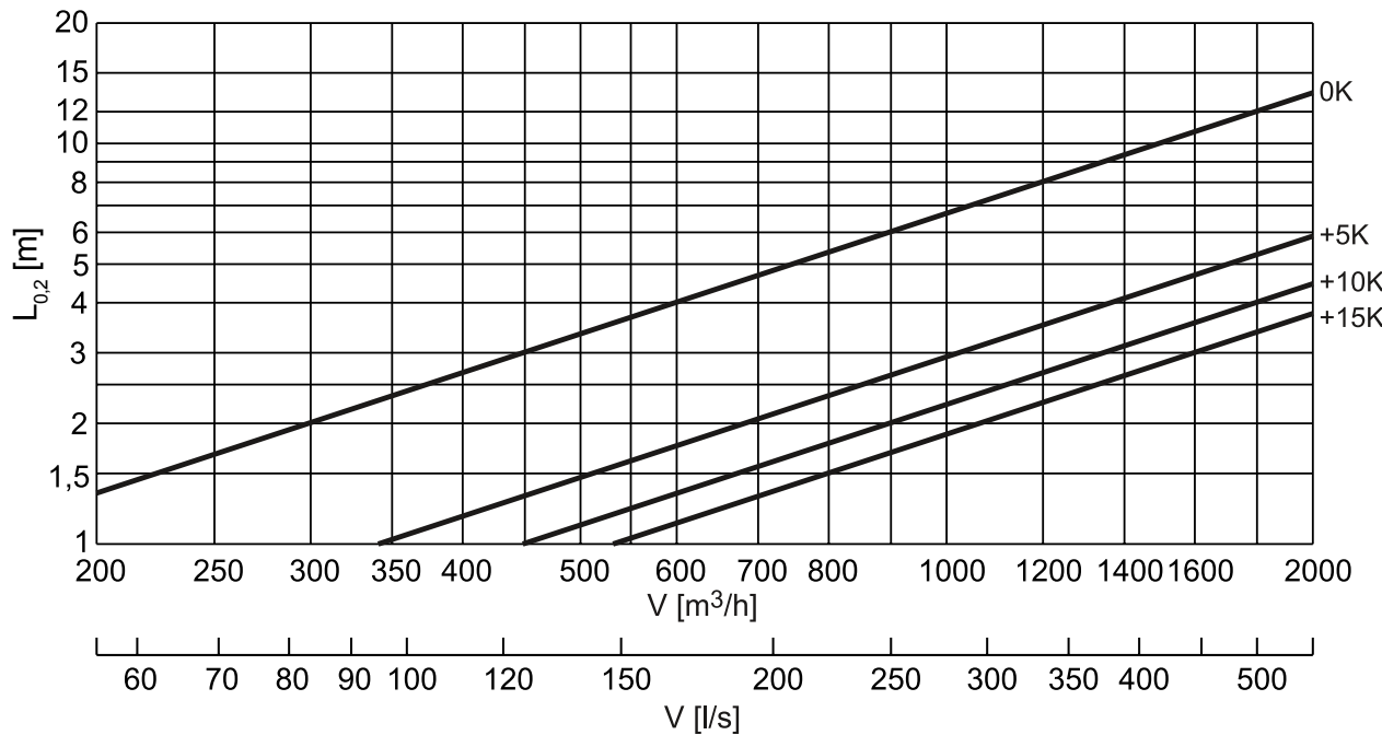
ODZA-31 – THROW LENGTH FOR HEATING FUNCTION (BLADES SET IN MIDDLE POSITION - AIR SUPPLY AT 45° ANGLE)
