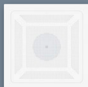
ATLAS-7 (HPKH)
