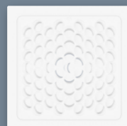
ARIES-1 (DYKH)
