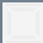
ATLAS-2 (RHKH)
