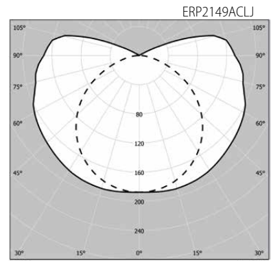
cd/klm – C0 - C180 --C90 - C270 94%
