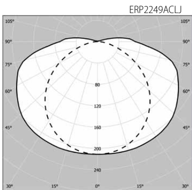
cd/klm – C0 - C180 --C90 - C270 89%
