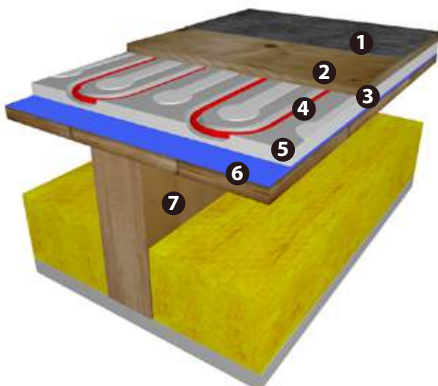
Fig. 22. Floor heating with Reflect insulated plates (EFCI Dry) on existing wooden floors
