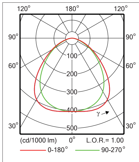
RC127V W30L120 OC
