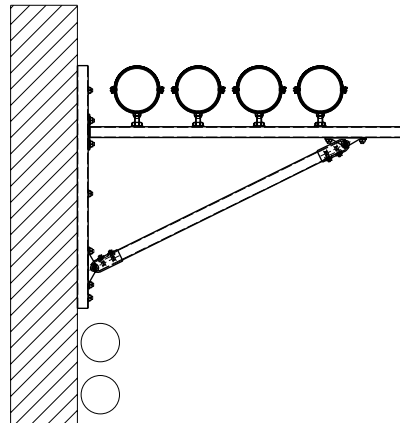
Pipes installed on a wall hanger bracket with diagonal strut
