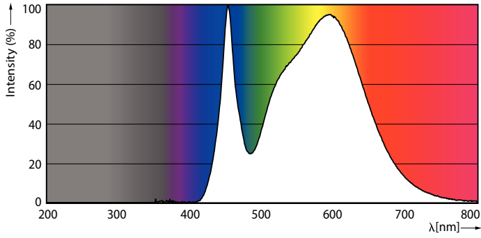
Spectral Power Distribution Colour - CorePro LED PLS 360D 3.5W 3CCT 2P G23
