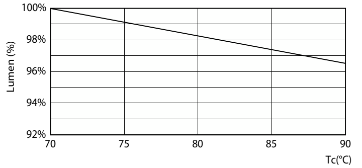
Lumen Maintenance Diagram - CorePro LED PLS 360D 3.5W 3CCT 2P G23
