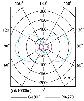
Light Distribution Diagram - CorePro LED PLS 360D 3.5W 3CCT 2P G23
