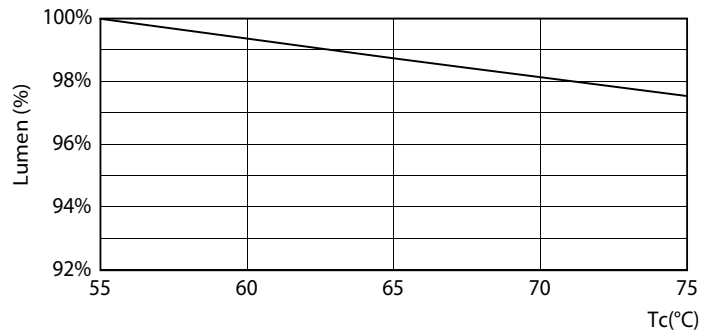
Lumen Maintenance Diagram - MAS LEDtube 1500mm UE 18.9W 840 T5 EELB
