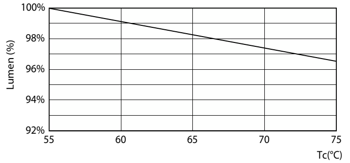
Lumen Maintenance Diagram - CorePro LEDtube 1200mm UO 17.5W 3CCT T8
