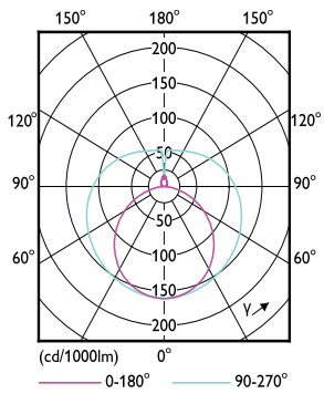
Light Distribution Diagram - CorePro LEDtube 1200mm UO 17.5W 3CCT T8
