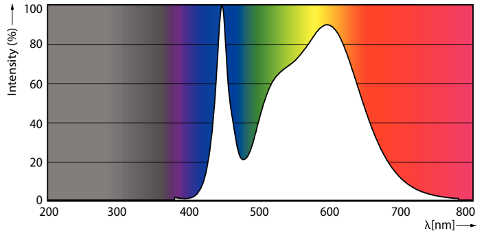
Spectral Power Distribution Colour - CorePro LEDtube 1200mm UO 17.5W 3CCT T8
