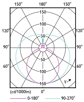
Light Distribution Diagram - CorePro LEDtube 600mm HO 7.7W 3CCT T8
