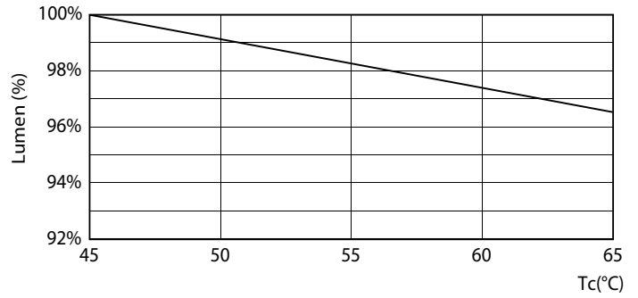
Lumen Maintenance Diagram - CorePro LEDtube 600mm HO 7.7W 3CCT T8
