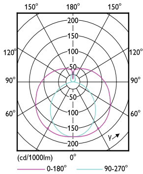
Light Distribution Diagram - MAS LEDtube VLE 1500mm 19.3W/23W 865 T8
