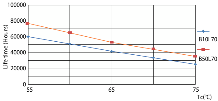
LifetimeVsTc
