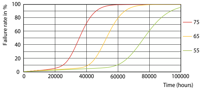
LEDtube-75K-5575-FailureRate-LED
