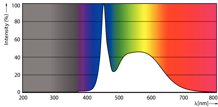
Spectral Power Distribution Colour - MAS LEDtube VLE 1500mm 19.3W/23W 865 T8
