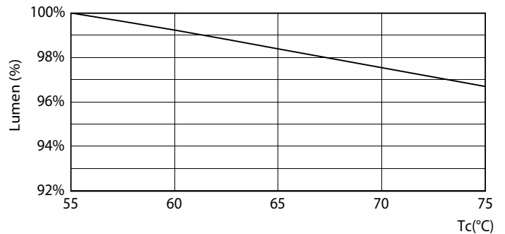
Lumen Maintenance Diagram - MAS LEDtube VLE 1500mm 19.3W/23W 865 T8
