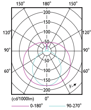
Light Distribution Diagram - MAS LEDtube VLE 1500mm 19.3W/23W 840 T8
