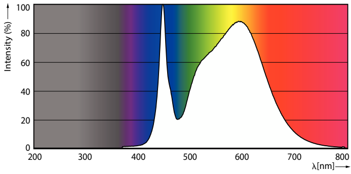
Spectral Power Distribution Colour - MAS LEDtube VLE 1500mm 19.3W/23W 840 T8
