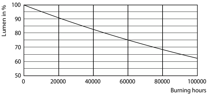
Lumen Maintenance Diagram - MAS LEDtube VLE 1500mm 19.3W/23W 840 T8
