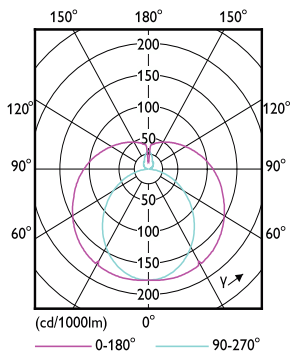
Light Distribution Diagram - MAS LEDtube VLE 1200mm 13.1W/15.5W 840T8
