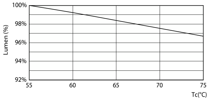
Lumen Maintenance Diagram - MAS LEDtube VLE 1200mm 13.1W/15.5W 840T8
