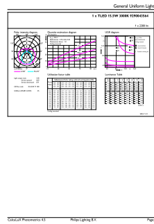
General uniform lighting - MAS LEDtube VLE 1200mm 13.1W/15.5W 830T8
