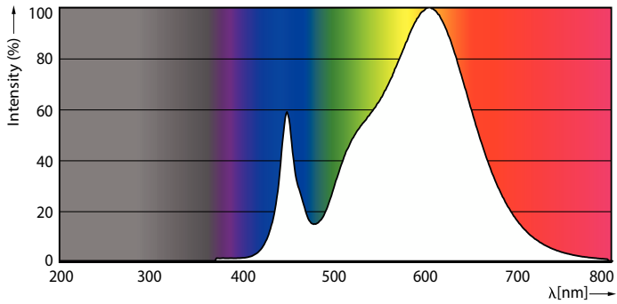
Spectral Power Distribution Colour - MAS LEDtube VLE 1200mm 13.1W/15.5W 830T8
