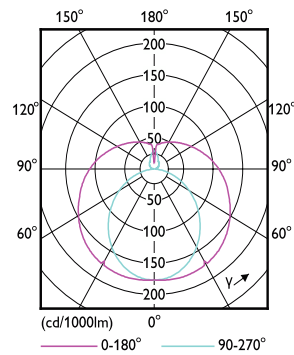
Light Distribution Diagram - MAS LEDtube VLE 1200mm 13.1W/15.5W 830T8
