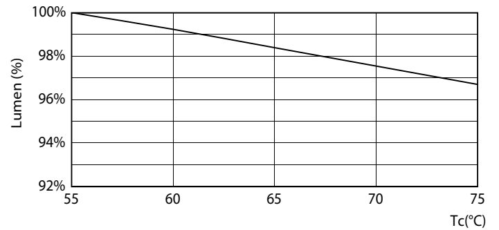
Lumen Maintenance Diagram - MAS LEDtube VLE 1200mm 13.1W/15.5W 830T8
