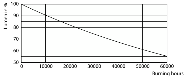
Lumen Maintenance Diagram - CorePro LED PLT HF/Mains 6.5W 830 4P
