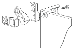
Wall mounting lugs fixing
