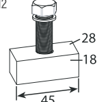
SYS-NPB12 (M12X30)
