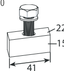
SYS-NPB12 (M12X30)
