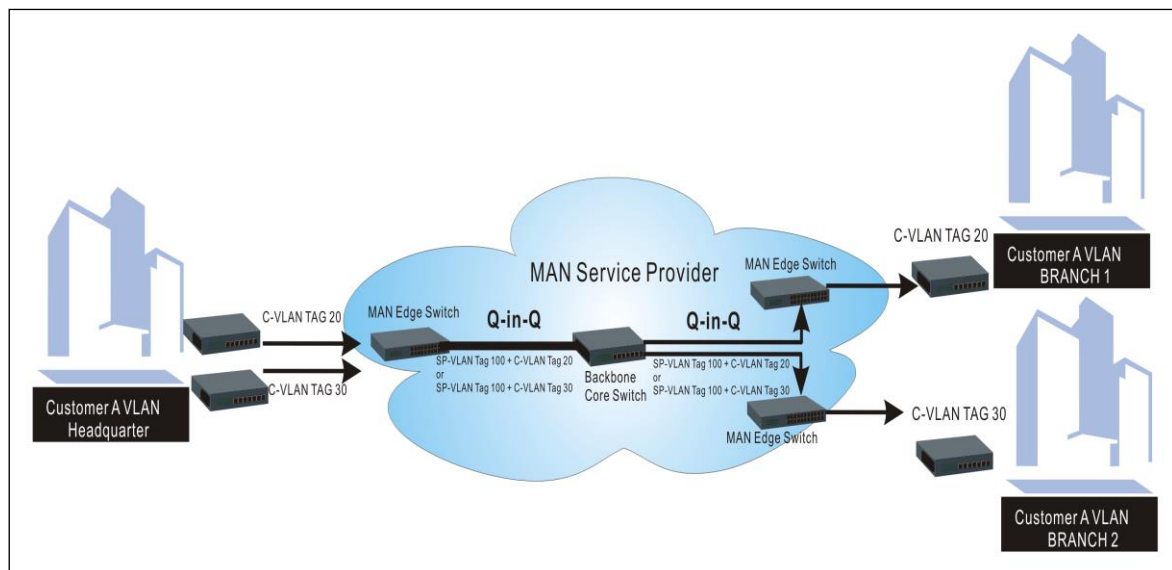
Q-in-Q Example
