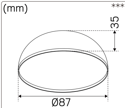
Accessory - Reflector
