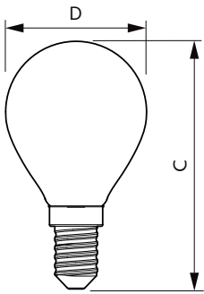
Candle P45 4.3-40W 470lm4000K E14NDClear
