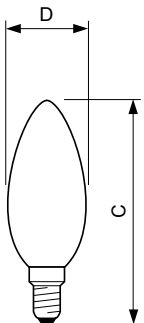
Candle B35 60W 806lm 6500K E14 NDFrosted
