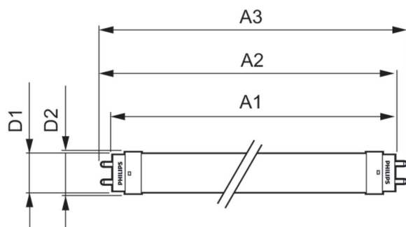
CorePro LEDtube 1200mm UO 21.5W 865 T8
