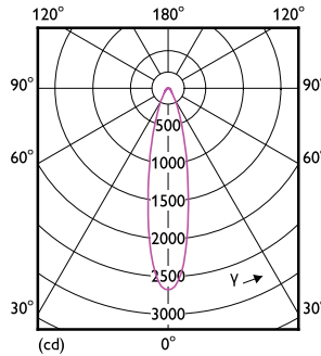
LEDspots MAS 9,5W PAR30S E27 840 25D
