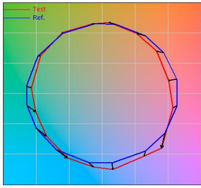
TM-30-15 Color Vector Graphic Rf=81 Rg=97
