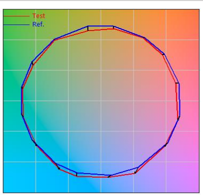
TM-30-15 Color Vector Graphic Rf=90 Rg=88
