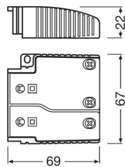
OT CABLE CLAMP B-STYLE LP
