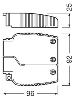
611986_OT CABLE CLAMP A-STYLE TL
