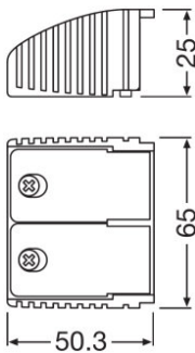
554789_OT CABLE CLAMP A-STYLE
