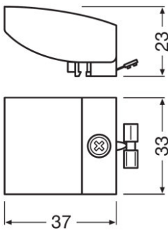
OT Cable clamp N-style
