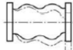
Lateral displacement
