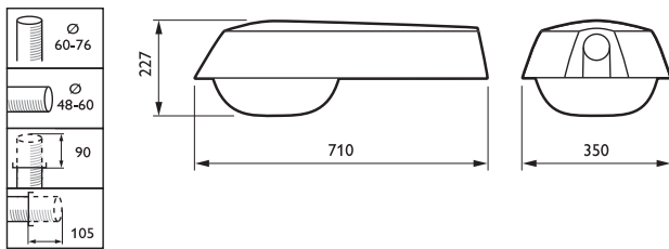
SGP100 SON-T100W II R-A-R ACF
