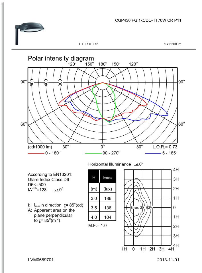
CGP430 FG 1xCDO-TT70W CR P11
