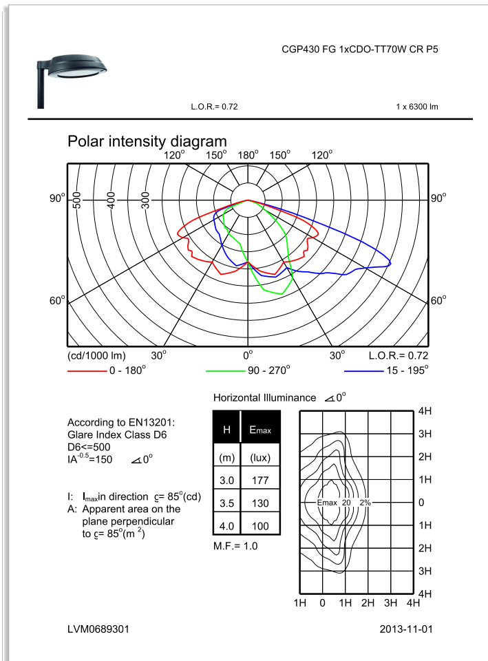
CGP430 FG 1xCDO-TT70W CR P5
