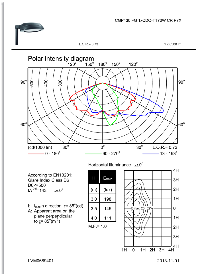
CGP430 FG 1xCDO-TT70W CR P7X
