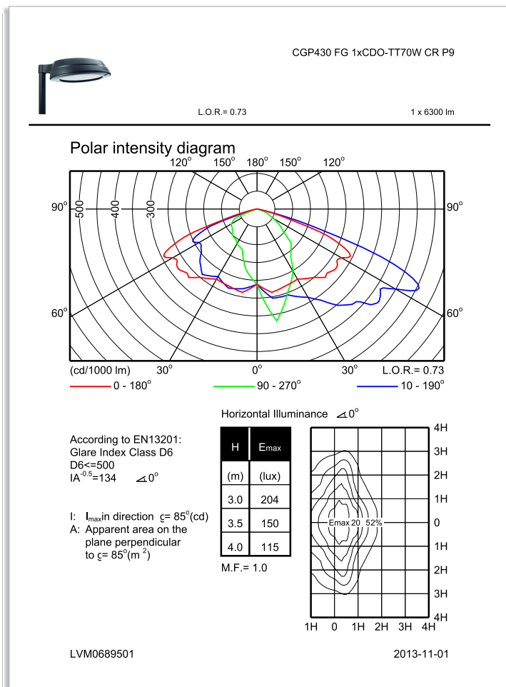
CGP430 FG 1xCDO-TT70W CR P9
