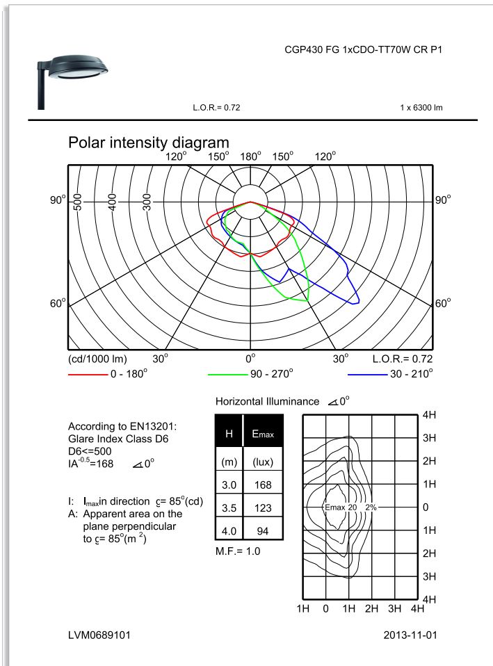
CGP430 FG 1xCDO-TT70W CR P1
