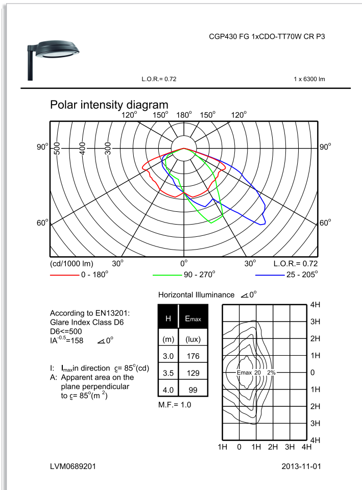
CGP430 FG 1xCDO-TT70W CR P3
