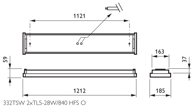
332TSW 2xTL5-28W/840 HFS O
