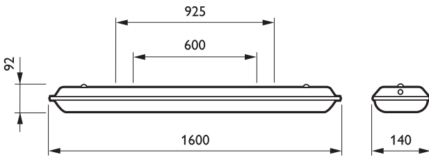
TCW215 2xTL-D58W/840 HFP KIT
