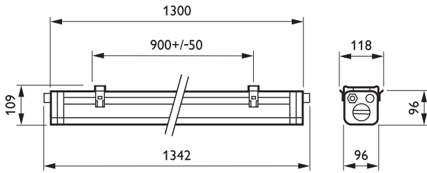
WT461C LED23S/840 PSU WB TW1 L1300
