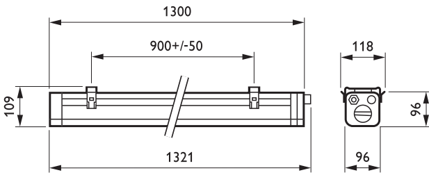
WT360C 2xTL5-54W/830 HFP C
